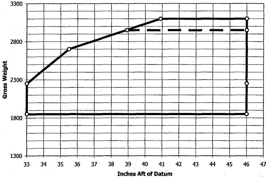
CG Inches Aft of Datum Envelope
